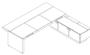
2550x2300xh: 730
