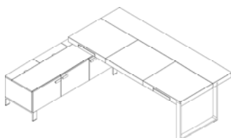
2550x2300xh: 730
