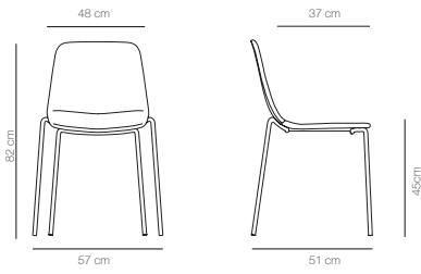
MAAL4P - Four legs base smooth upholstery
