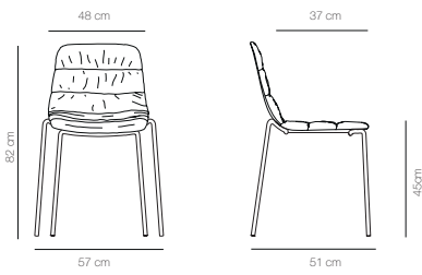
MAA4P - Four legs base soft upholstery
