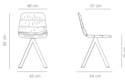
MAA - Swivel base soft upholstery
